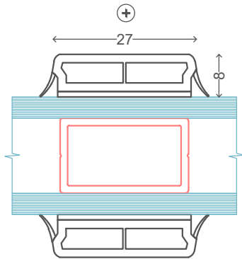
⊖ Standard PVC bars Glued on both sides 27mm + Duplex 2 layer glass
