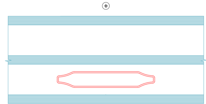
⊖ Bars inside the glass 45mm 3 layer glass
