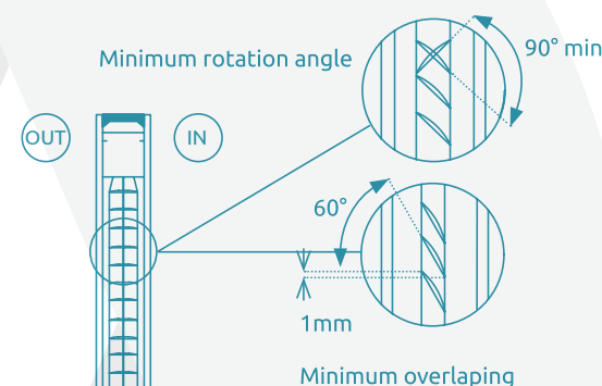
Fig. 16 Overlapping of slats.
