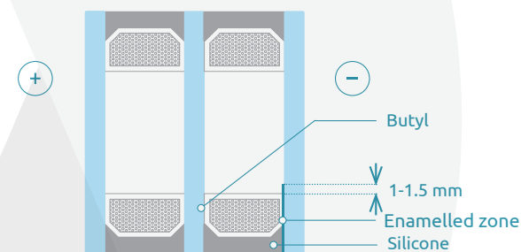
Fig. 22 Enamel zone for insulating glass units intended for bonded glazing.
