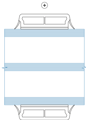
⊖ Standard PVC bars Glued on both sides 27mm 3 layer glass
