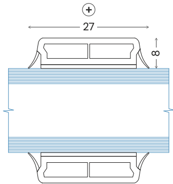
⊖ Standard PVC bars Glued on both sides 27mm 2 layer glass
